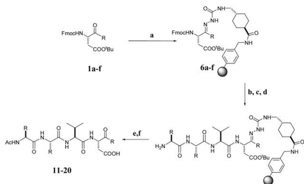
Figure 5. Reagents and conditions: (a) AcOH, THF, solid support 8 ; (b) 20% piperidine in DMF, rt, 30 min; (c) Fmoc-(AA) n -OH, HATU, DIEA, DMF, rt, 2 h; (d) repeat steps (b), (c), (b) until P 4 is attached; (e) acetylimidazole, DMF, 1 h; (f) TFA/H 2 O (9:1), 30 min. Steps (b), (c), and (d) are performed on PepSynthesizer.
